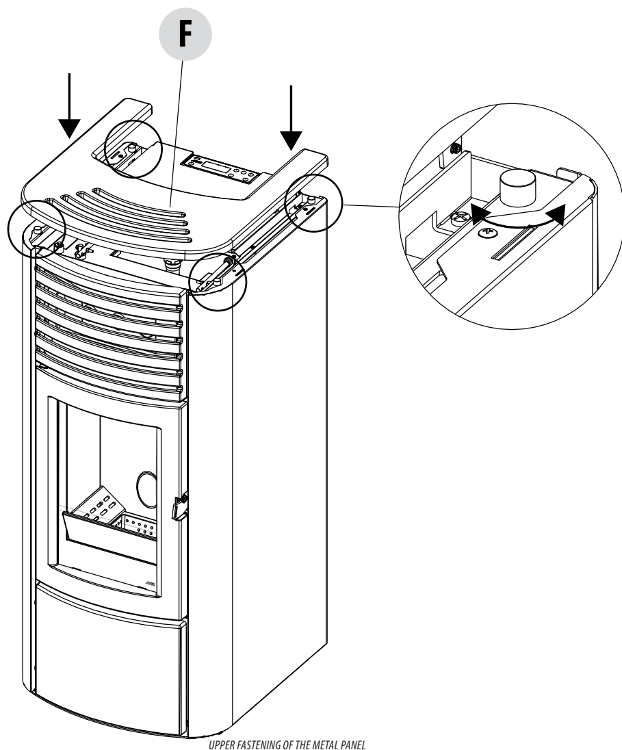
UPPER FASTENING OF THE METAL PANEL
